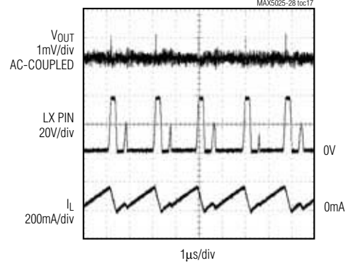
MAX5026, V_{CC} = 5V , V_{OUT} = 30V , I_{LOAD} = 4mA . CIRCUIT OF FIGURE 3
